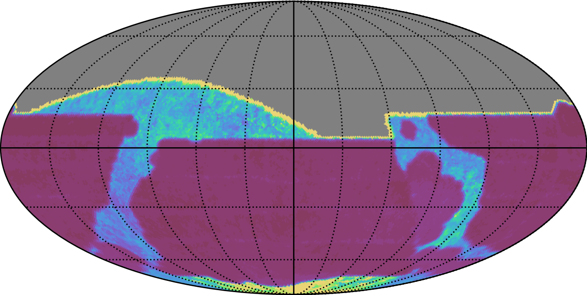
roll_uniform_early_half_mjdp67_v3.4_10yrs All sky all bands: Median Inter-Night Gap
