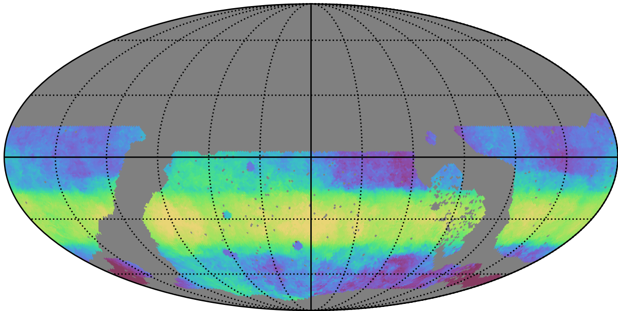
roll_uniform_early_half_mjdp67_v3.4_10yrs WFD i band: Median HA
