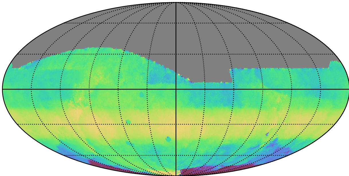
roll_uniform_early_half_mjdp67_v3.4_10yrs All sky i band: Median HA
