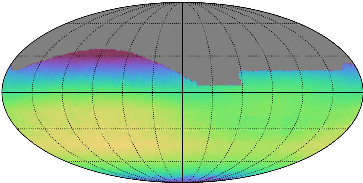
roll_uniform_early_half_mjdp67_v3.4_10yrs All sky i band: Max skyBrightness
