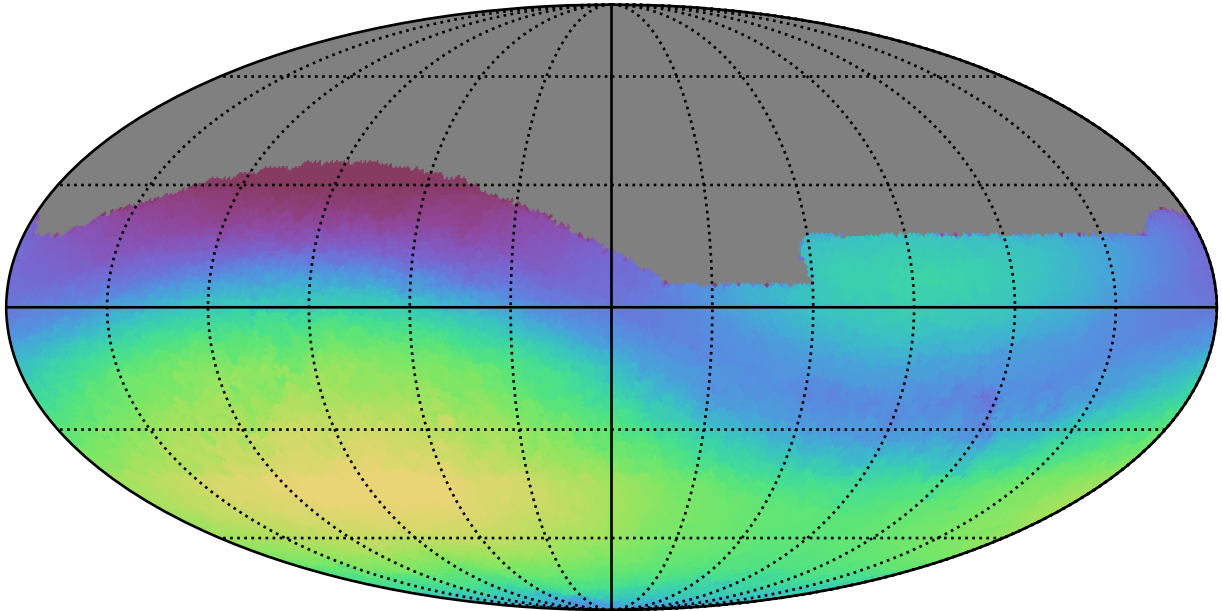
roll_uniform_early_half_mjdp67_v3.4_10yrs All sky g band: Max skyBrightness
