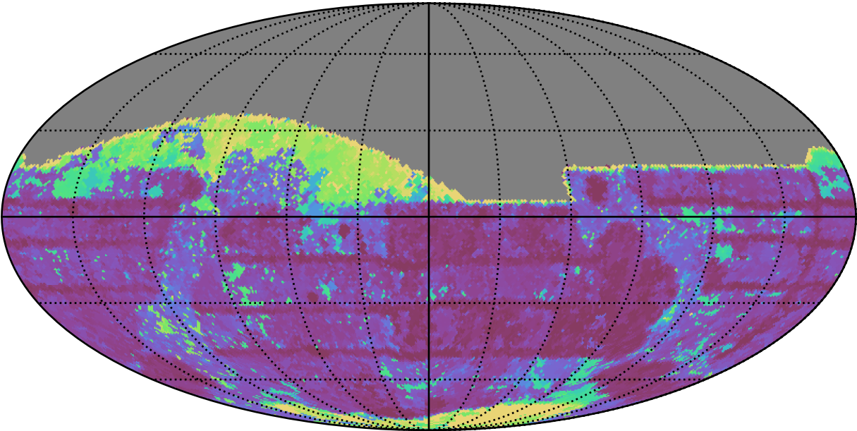
roll_uniform_early_half_mjdp67_v3.4_10yrs All sky z band: Max Inter-Night Gap
