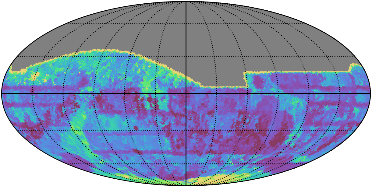
roll_uniform_early_half_mjdp67_v3.4_10yrs All sky all bands: Max Inter-Night Gap
