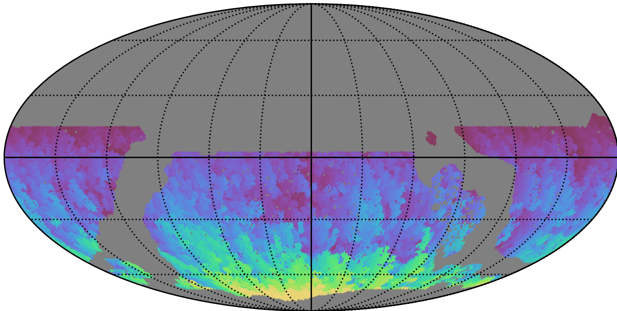
roll_uniform_early_half_mjdp67_v3.4_10yrs WFD y band: Max HA
