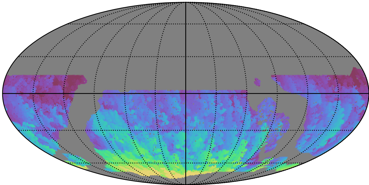
roll_uniform_early_half_mjdp67_v3.4_10yrs WFD r band: Max HA
