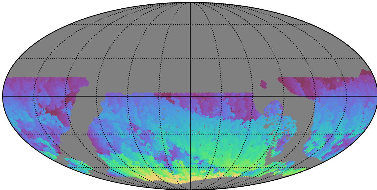
roll_uniform_early_half_mjdp67_v3.4_10yrs WFD i band: Max HA
