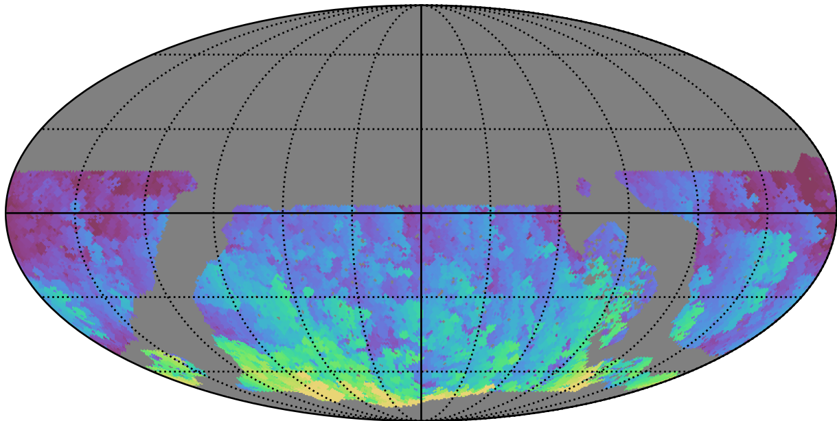
roll_uniform_early_half_mjdp67_v3.4_10yrs WFD g band: Max HA
