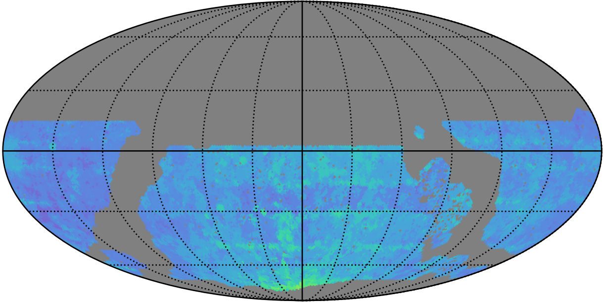
roll_uniform_early_half_mjdp67_v3.4_10yrs WFD y band: 80thPercentile Season Length
