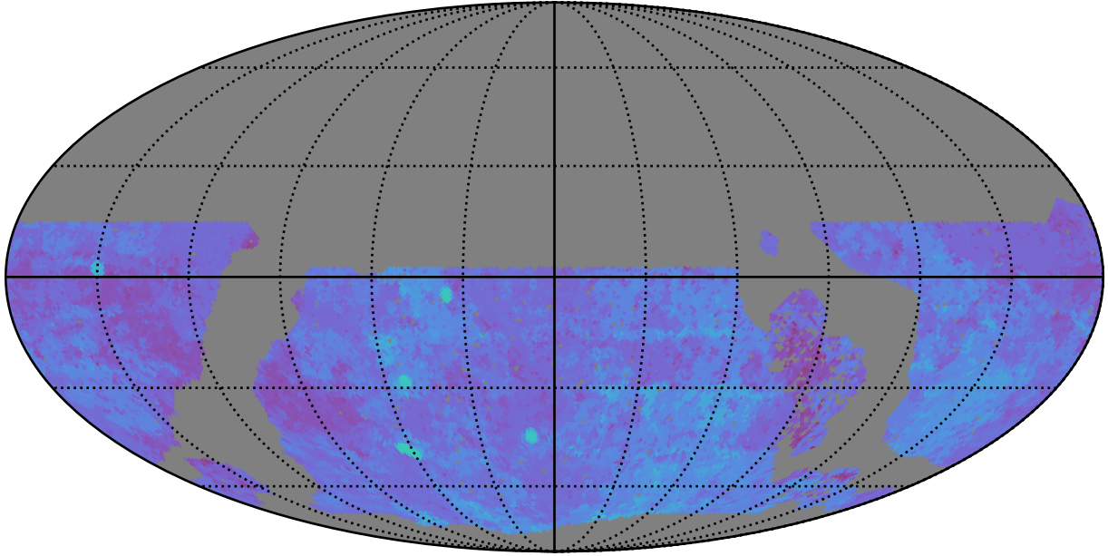
roll_uniform_early_half_mjdp67_v3.4_10yrs WFD u band: 80thPercentile Season Length
