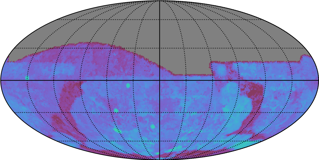
roll_uniform_early_half_mjdp67_v3.4_10yrs All sky g band: 80thPercentile Season Length
