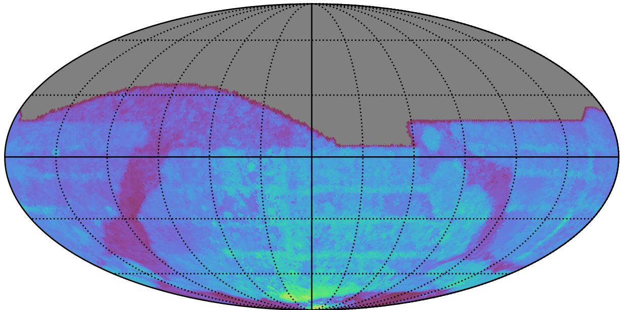
roll_uniform_early_half_mjdp67_v3.4_10yrs All sky all bands: 80thPercentile Season Length
