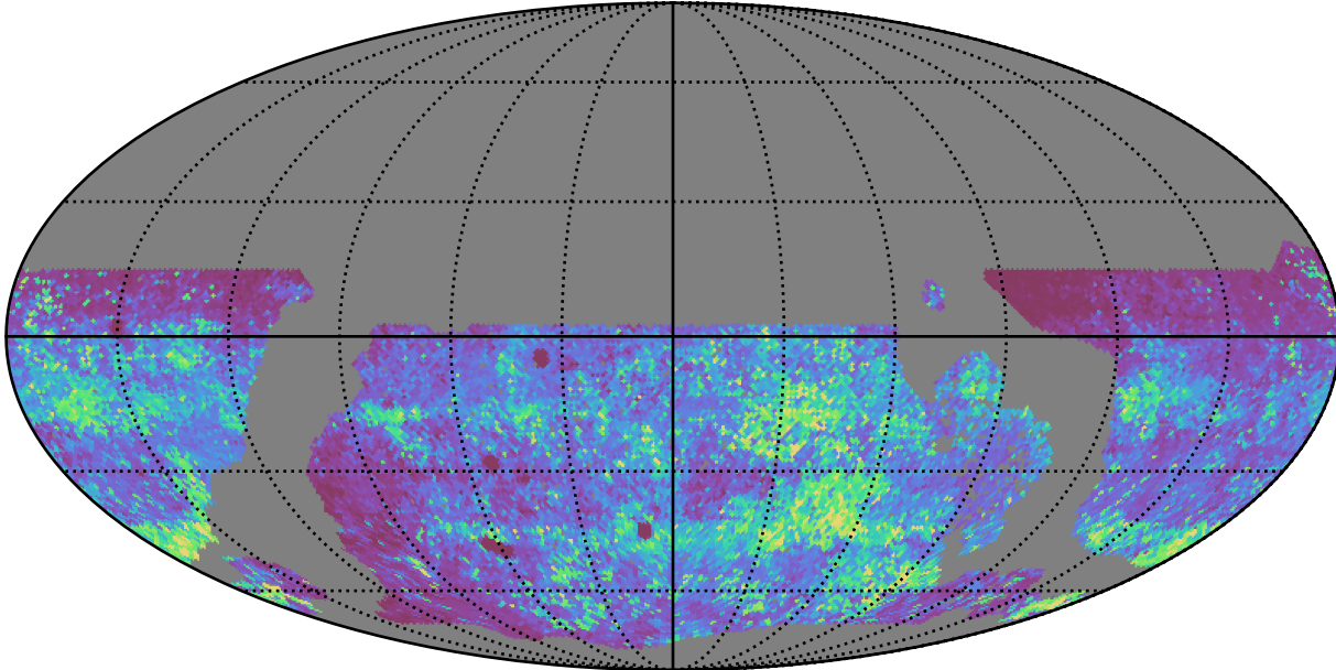
roll_uniform_early_half_mjdp67_v3.4_10yrs WFD zy bands: 75th Percentile Intranight Timespan
