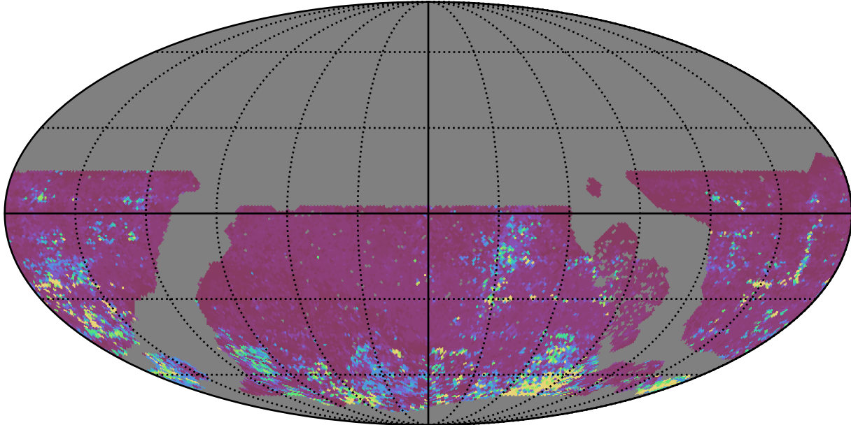
roll_uniform_early_half_mjdp67_v3.4_10yrs WFD z band: 75th Percentile Intranight Timespan
