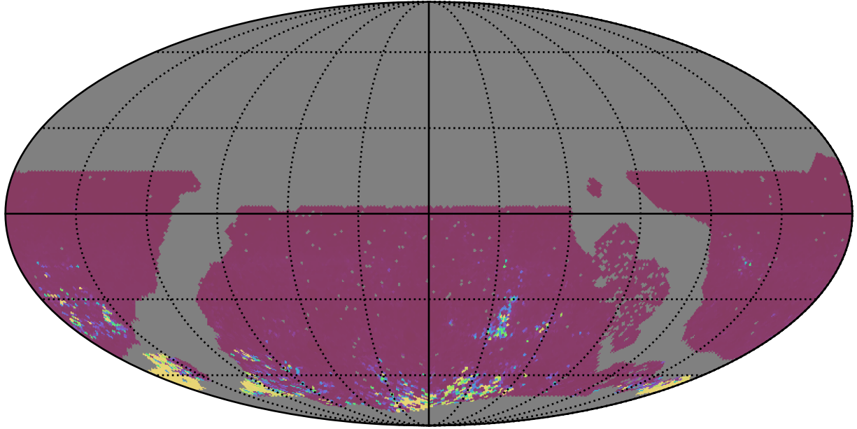
roll_uniform_early_half_mjdp67_v3.4_10yrs WFD ri bands: 75th Percentile Intranight Timespan
