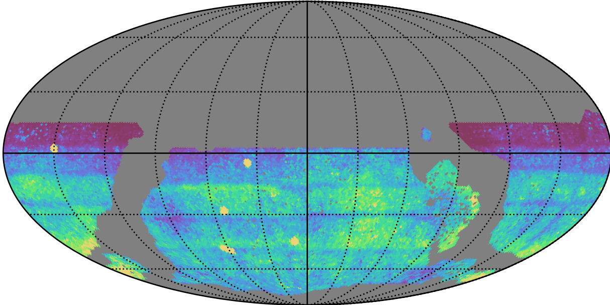
roll_uniform_early_half_mjdp67_v3.4_10yrs WFD all bands: 75th Percentile Intranight Timespan
