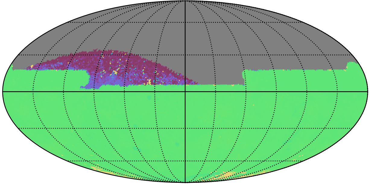
roll_uniform_early_half_mjdp67_v3.4_10yrs All sky zy bands: 75th Percentile Intranight Timespan
