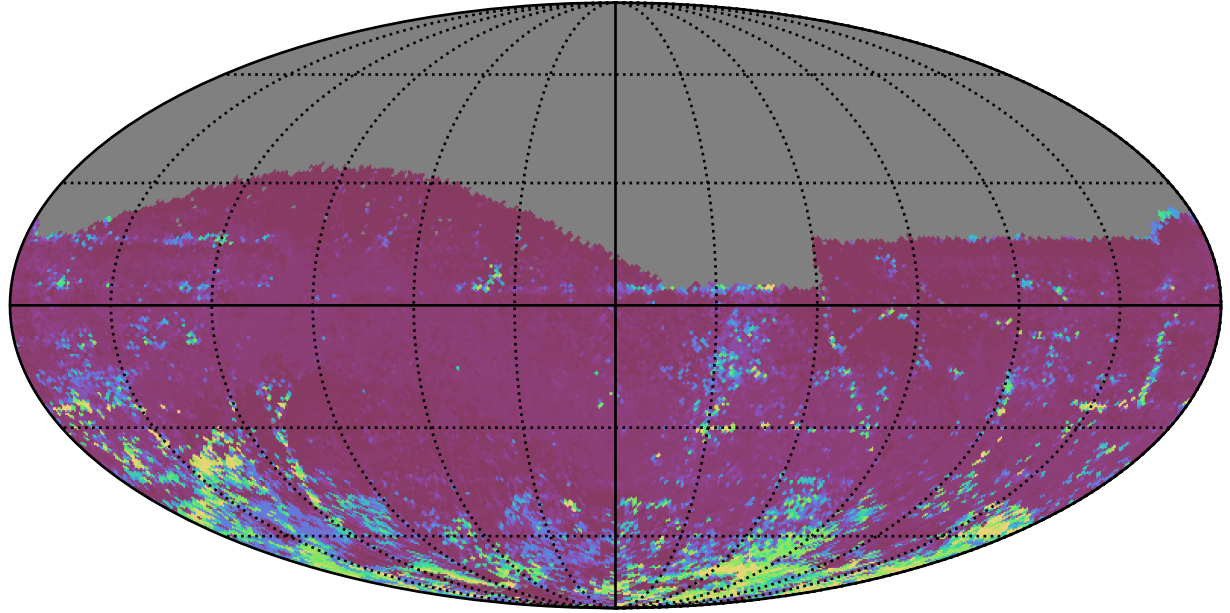
roll_uniform_early_half_mjdp67_v3.4_10yrs All sky z band: 75th Percentile Intranight Timespan
