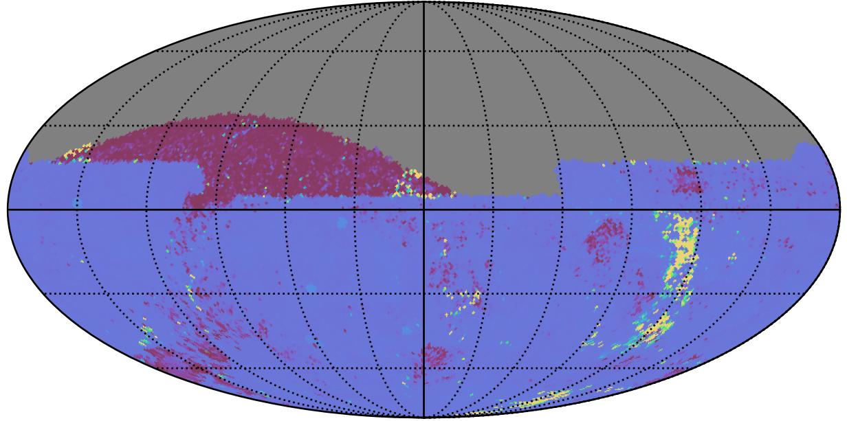
roll_uniform_early_half_mjdp67_v3.4_10yrs All sky ug bands: 75th Percentile Intranight Timespan
