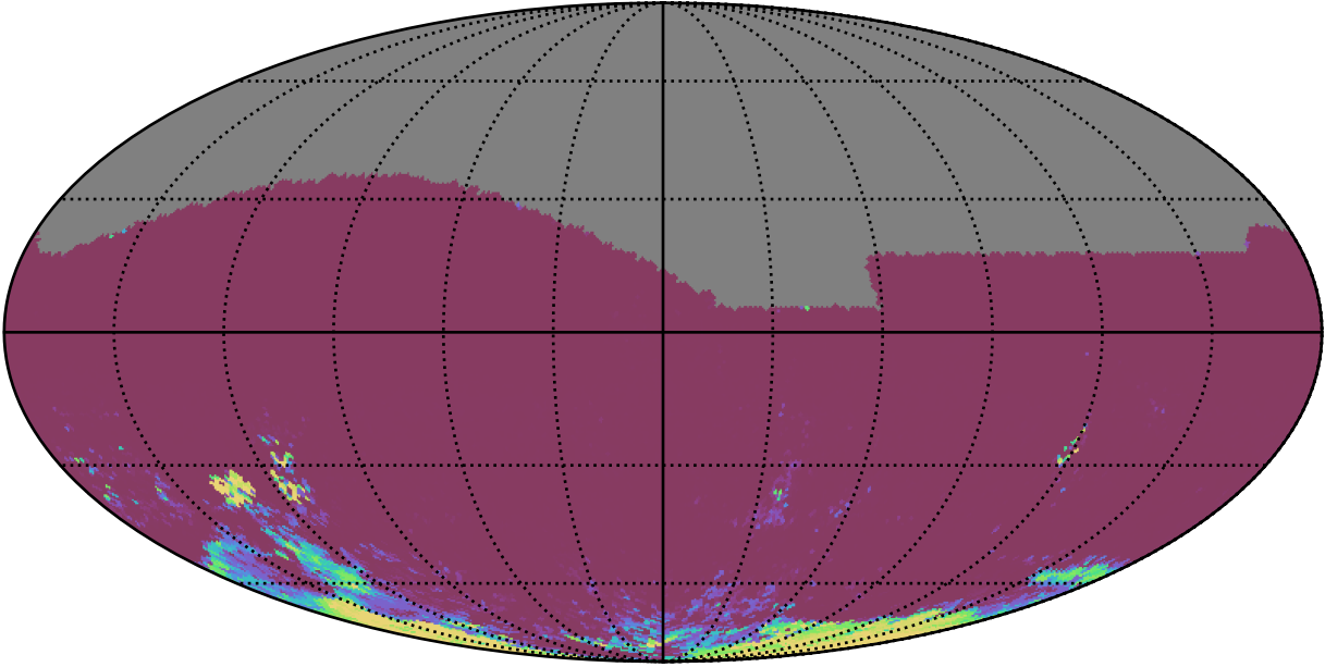
roll_uniform_early_half_mjdp67_v3.4_10yrs All sky ri bands: 75th Percentile Intranight Timespan
