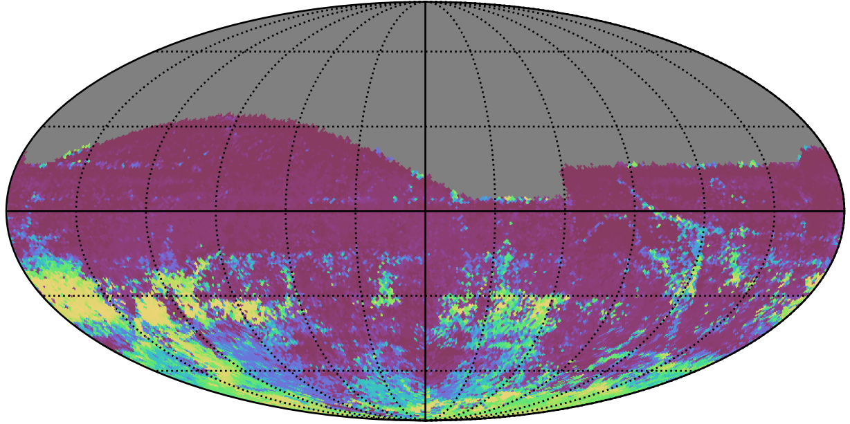
roll_uniform_early_half_mjdp67_v3.4_10yrs All sky r band: 75th Percentile Intranight Timespan
