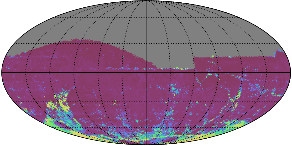
roll_uniform_early_half_mjdp67_v3.4_10yrs All sky i band: 75th Percentile Intranight Timespan
