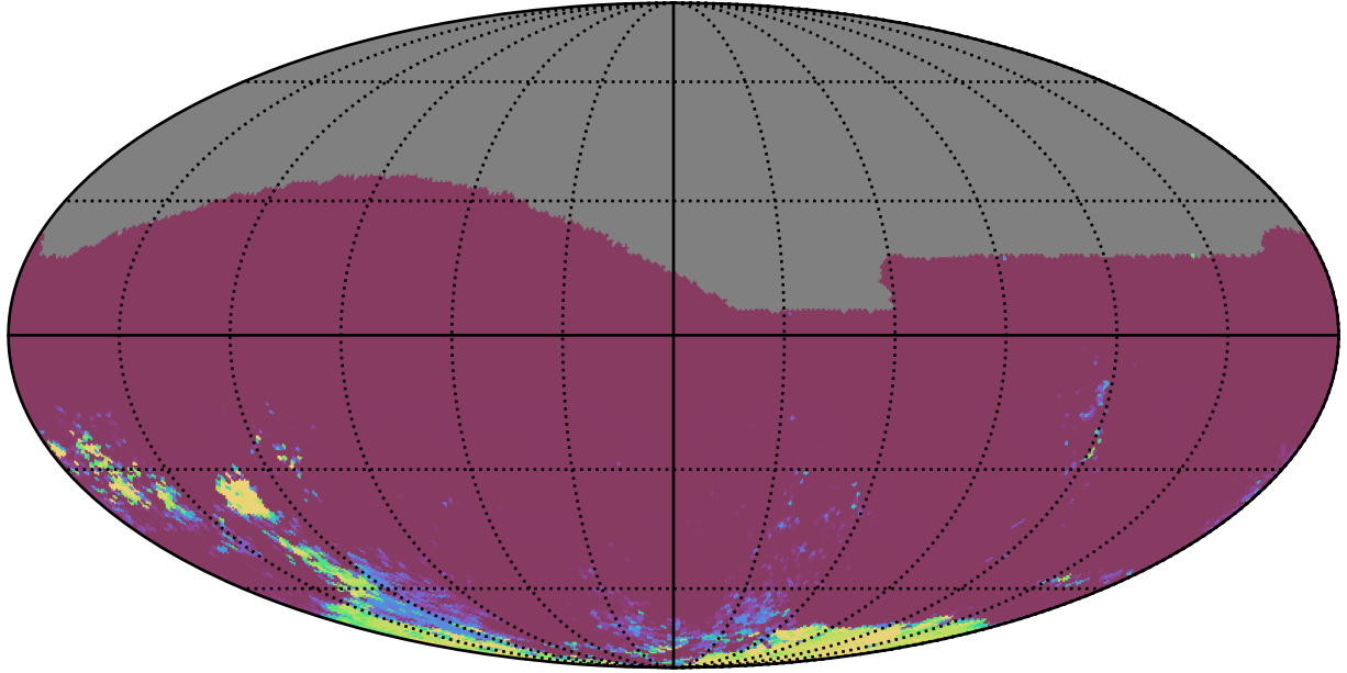
roll_uniform_early_half_mjdp67_v3.4_10yrs All sky gr bands: 75th Percentile Intranight Timespan
