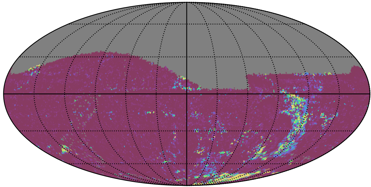
roll_uniform_early_half_mjdp67_v3.4_10yrs All sky g band: 75th Percentile Intranight Timespan
