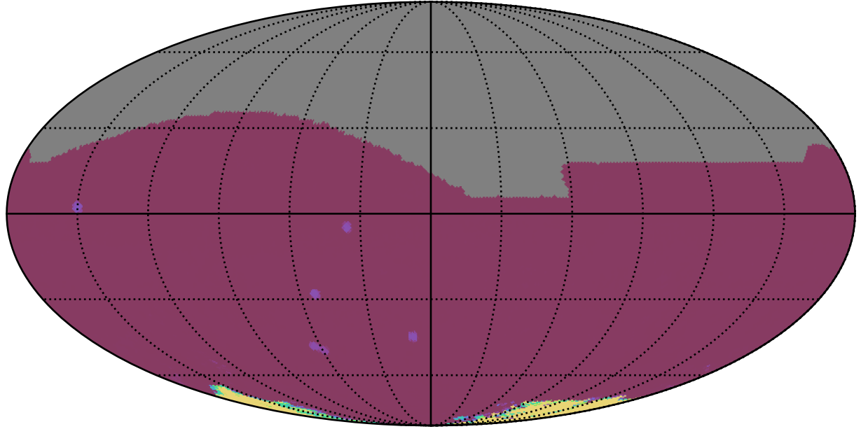
roll_uniform_early_half_mjdp67_v3.4_10yrs All sky all bands: 75th Percentile Intranight Timespan
