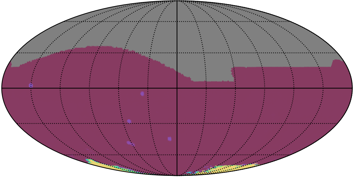
roll_uniform_early_half_mjdp67_v3.4_10yrs All sky: 75th Percentile Intranight Timespan
