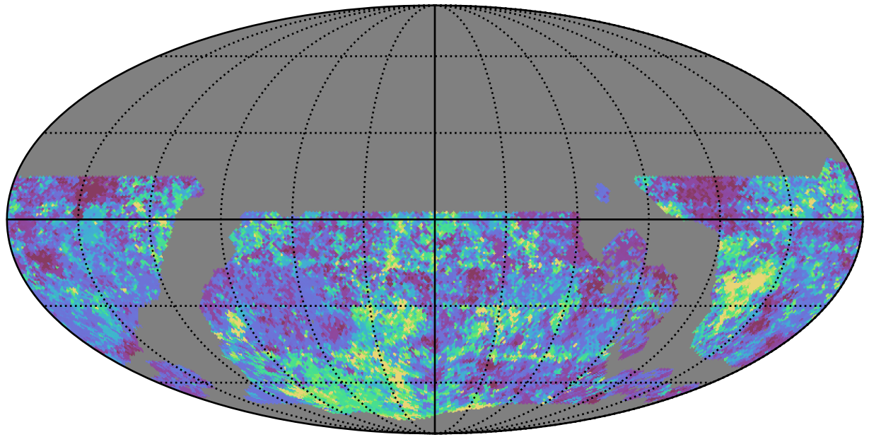
roll_uniform_early_half_mjdp67_v3.4_10yrs WFD g band: 20thPercentile Inter-Night Gap
