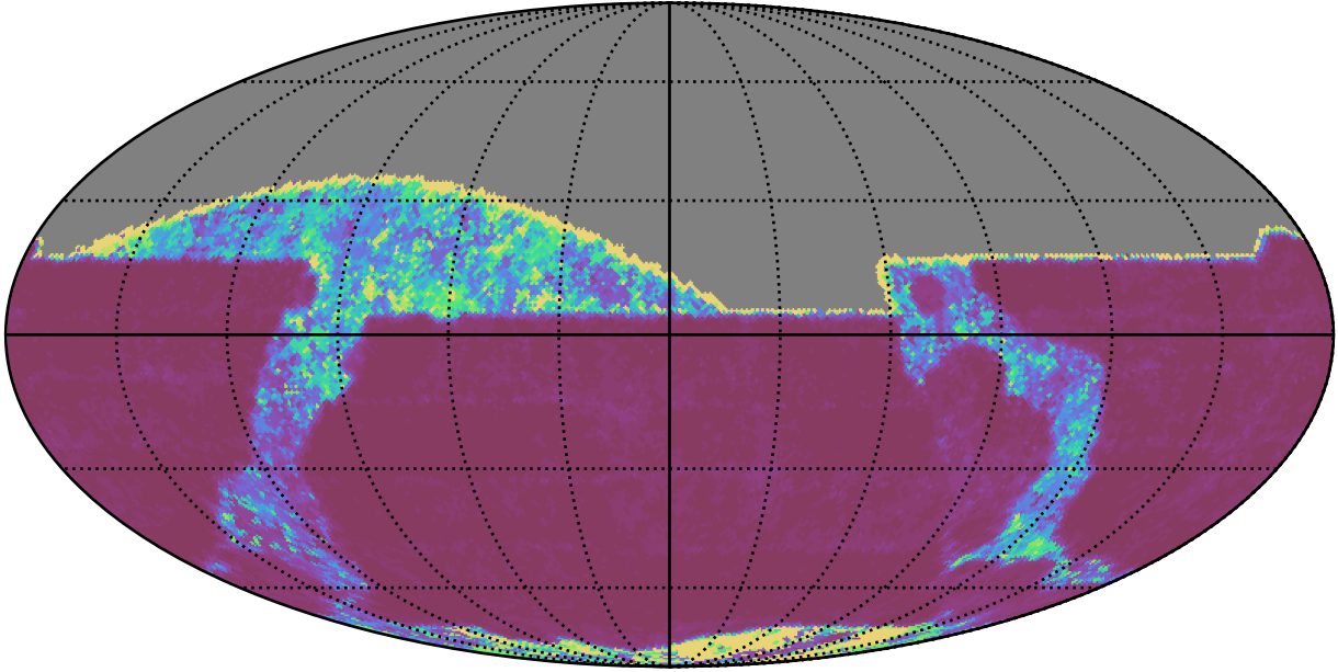
roll_uniform_early_half_mjdp67_v3.4_10yrs All sky z band: 20thPercentile Inter-Night Gap
