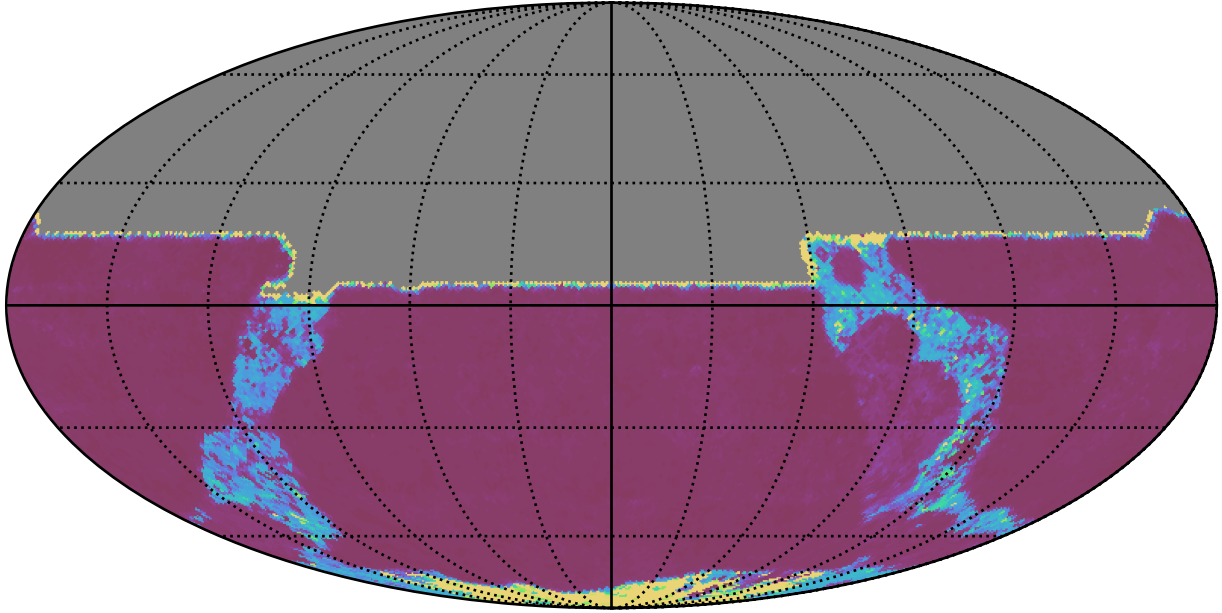
roll_uniform_early_half_mjdp67_v3.4_10yrs All sky y band: 20thPercentile Inter-Night Gap
