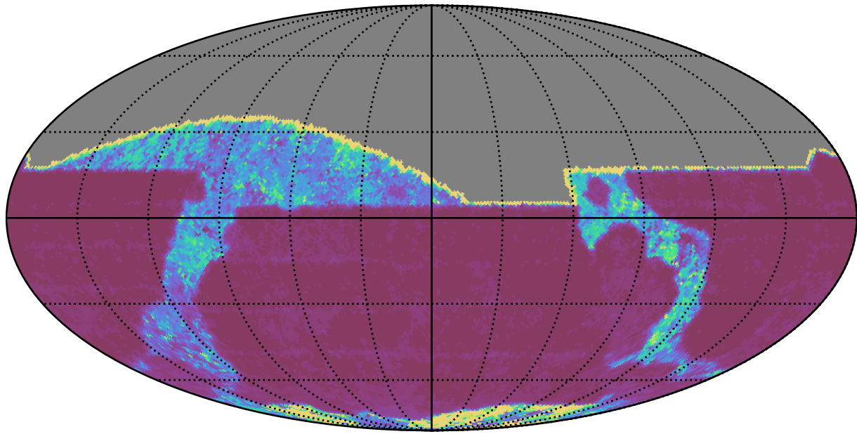
roll_uniform_early_half_mjdp67_v3.4_10yrs All sky i band: 20thPercentile Inter-Night Gap
