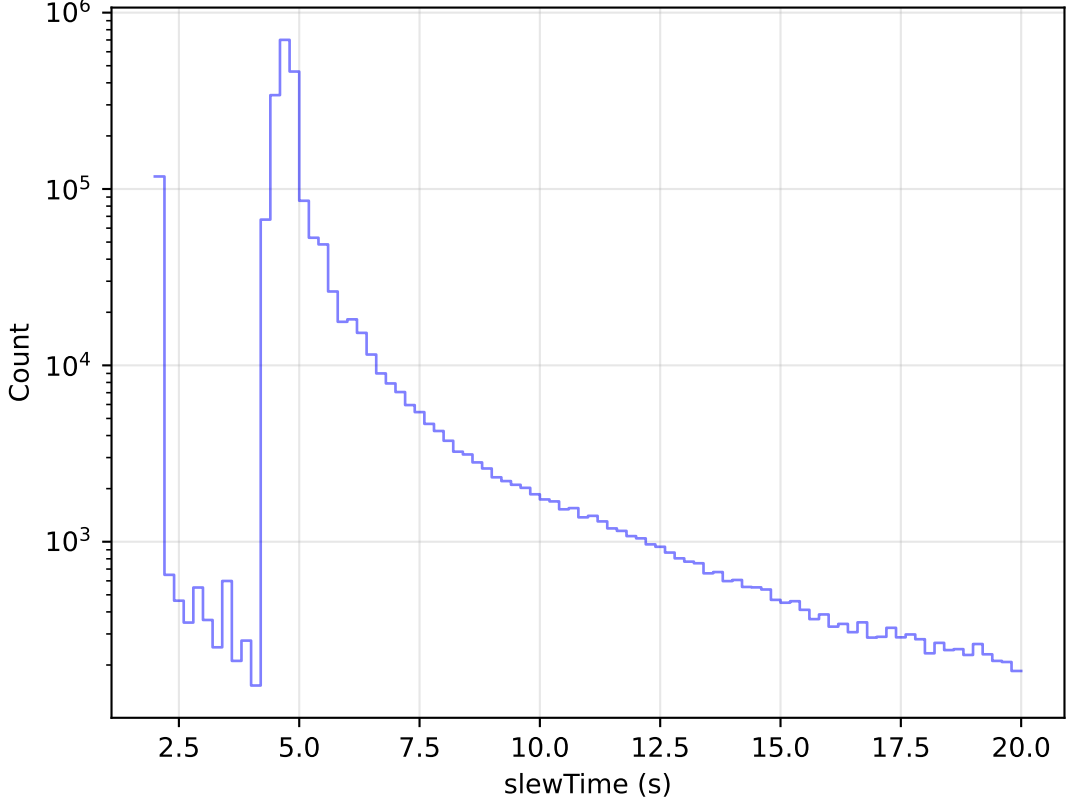
roll_uniform_early_half_mjdp67_v3.4_10yrs All visits: Zoom Slew Time Histogram
