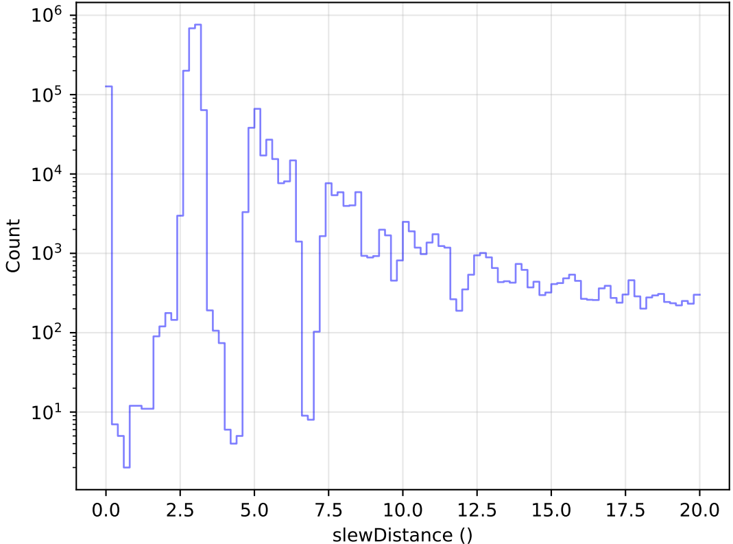
roll_uniform_early_half_mjdp67_v3.4_10yrs All visits: Zoom Slew Distance Histogram
