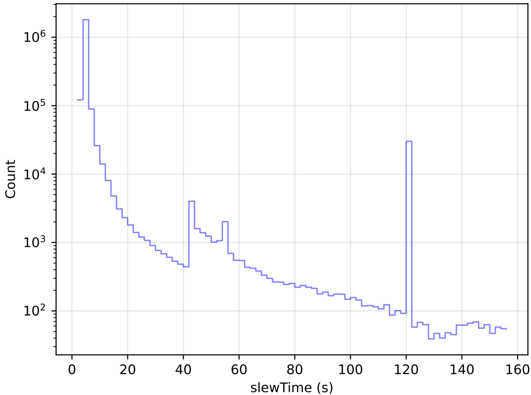
roll_uniform_early_half_mjdp67_v3.4_10yrs All visits: Slew Time Histogram
