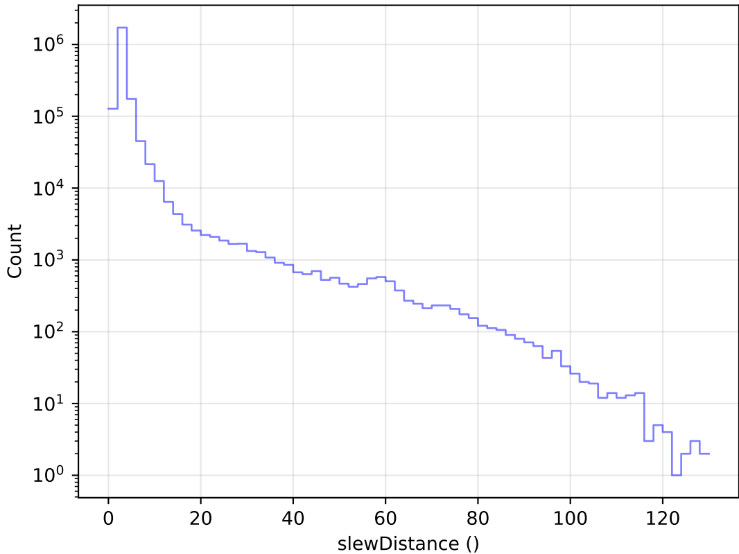
roll_uniform_early_half_mjdp67_v3.4_10yrs All visits: Slew Distance Histogram
