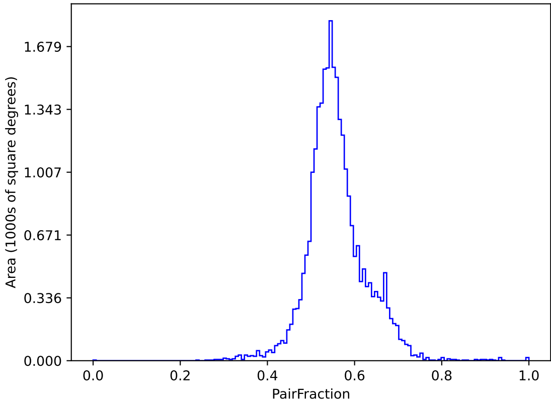
roll_uniform_early_half_mjdp67_v3.4_10yrs (g or r or i): PairFraction
