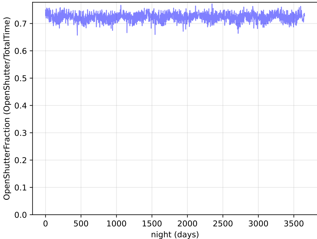
roll_uniform_early_half_mjdp67_v3.4_10yrs : OpenShutterFraction
