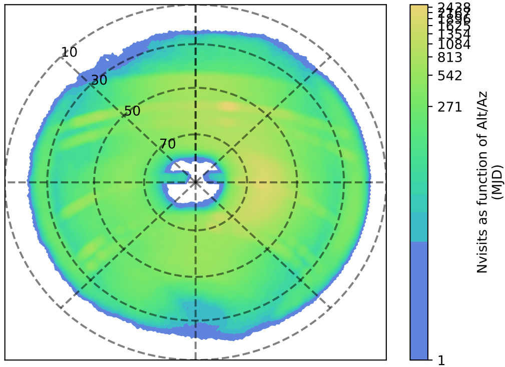
roll_uniform_early_half_mjdp67_v3.4_10yrs z: Nvisits as function of Alt/Az
