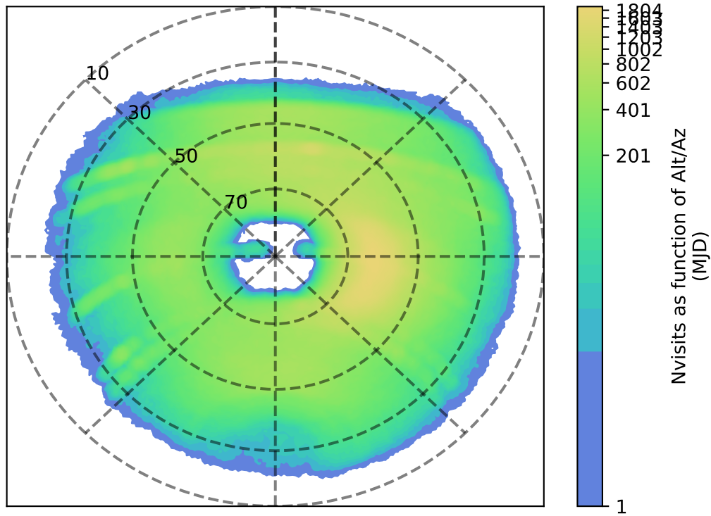
roll_uniform_early_half_mjdp67_v3.4_10yrs y: Nvisits as function of Alt/Az
