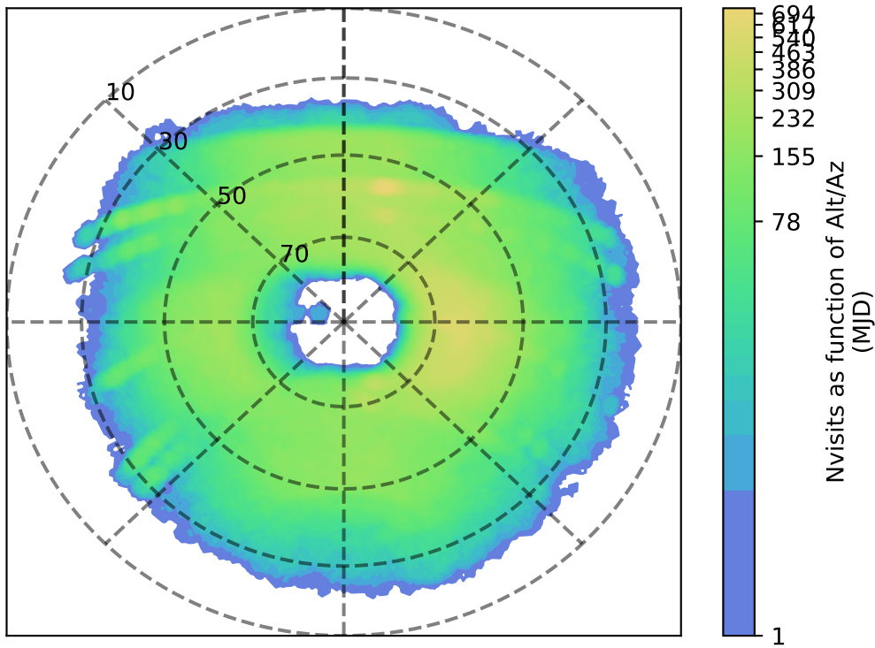
roll_uniform_early_half_mjdp67_v3.4_10yrs u: Nvisits as function of Alt/Az
