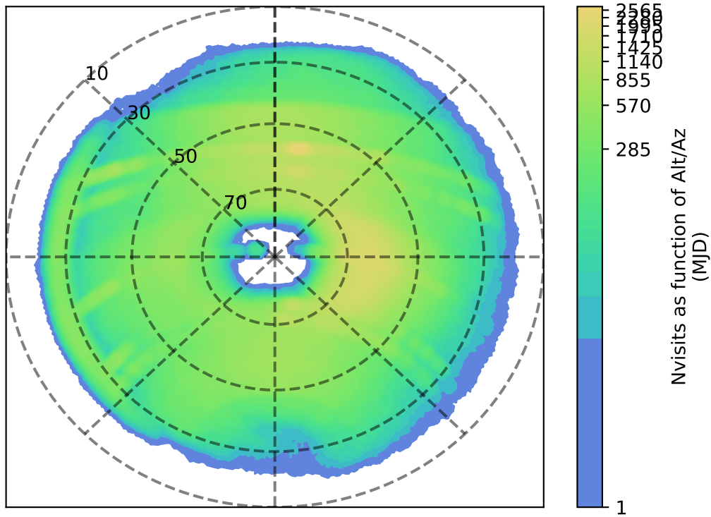
roll_uniform_early_half_mjdp67_v3.4_10yrs r: Nvisits as function of Alt/Az
