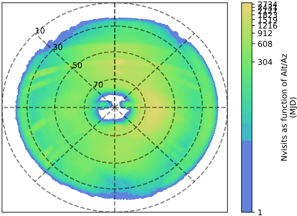
roll_uniform_early_half_mjdp67_v3.4_10yrs i: Nvisits as function of Alt/Az
