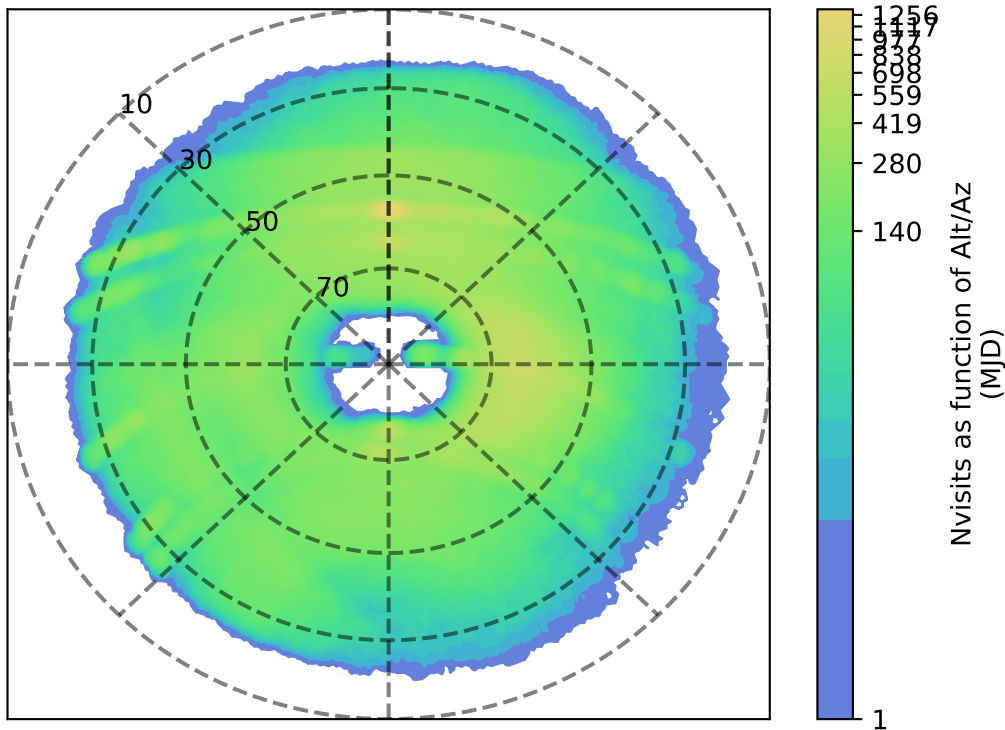
roll_uniform_early_half_mjdp67_v3.4_10yrs g: Nvisits as function of Alt/Az
