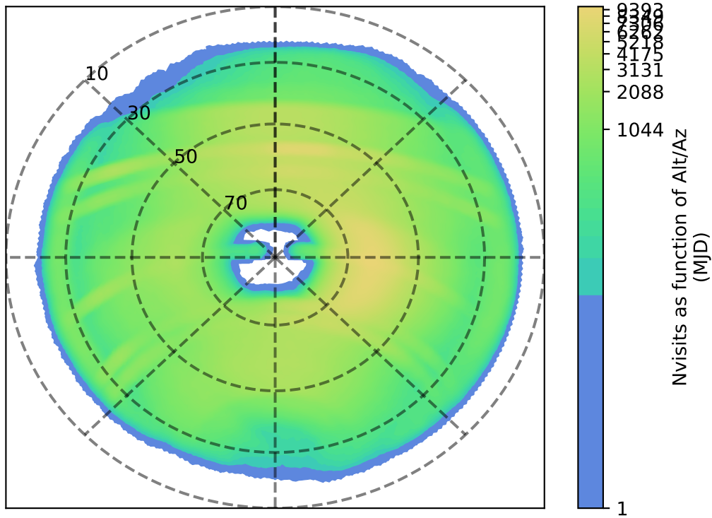
roll_uniform_early_half_mjdp67_v3.4_10yrs : Nvisits as function of Alt/Az
