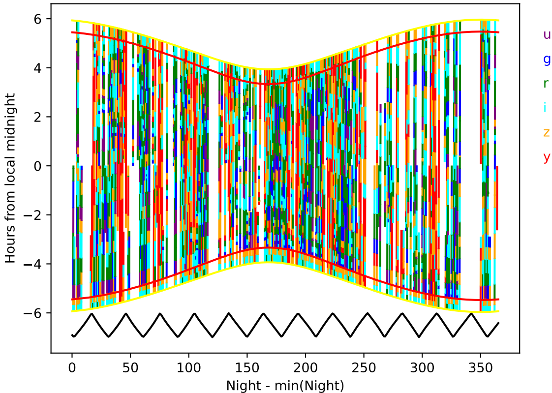
roll_uniform_early_half_mjdp67_v3.4_10yrs year 7-8: Hourglass
