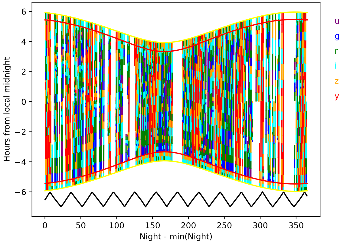
roll_uniform_early_half_mjdp67_v3.4_10yrs year 5-6: Hourglass
