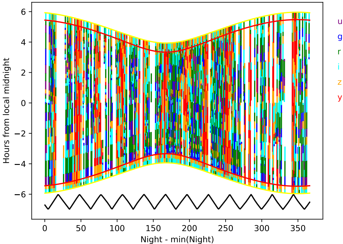
roll_uniform_early_half_mjdp67_v3.4_10yrs year 4-5: Hourglass
