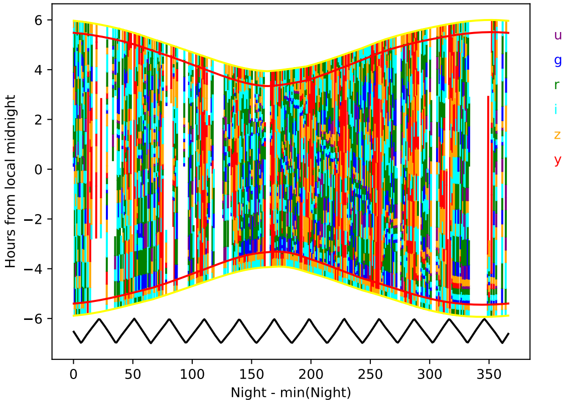
roll_uniform_early_half_mjdp67_v3.4_10yrs year 1-2: Hourglass
